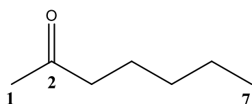
2-eptanone
