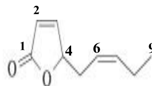
(6Z)-2,6-nonadien-4-olide
